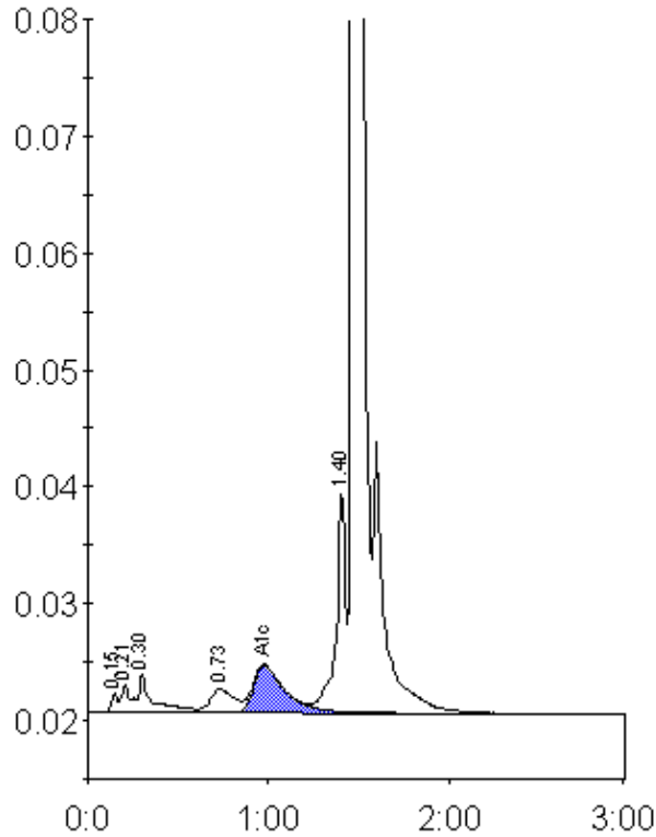
Peak table - ID: 10522832
